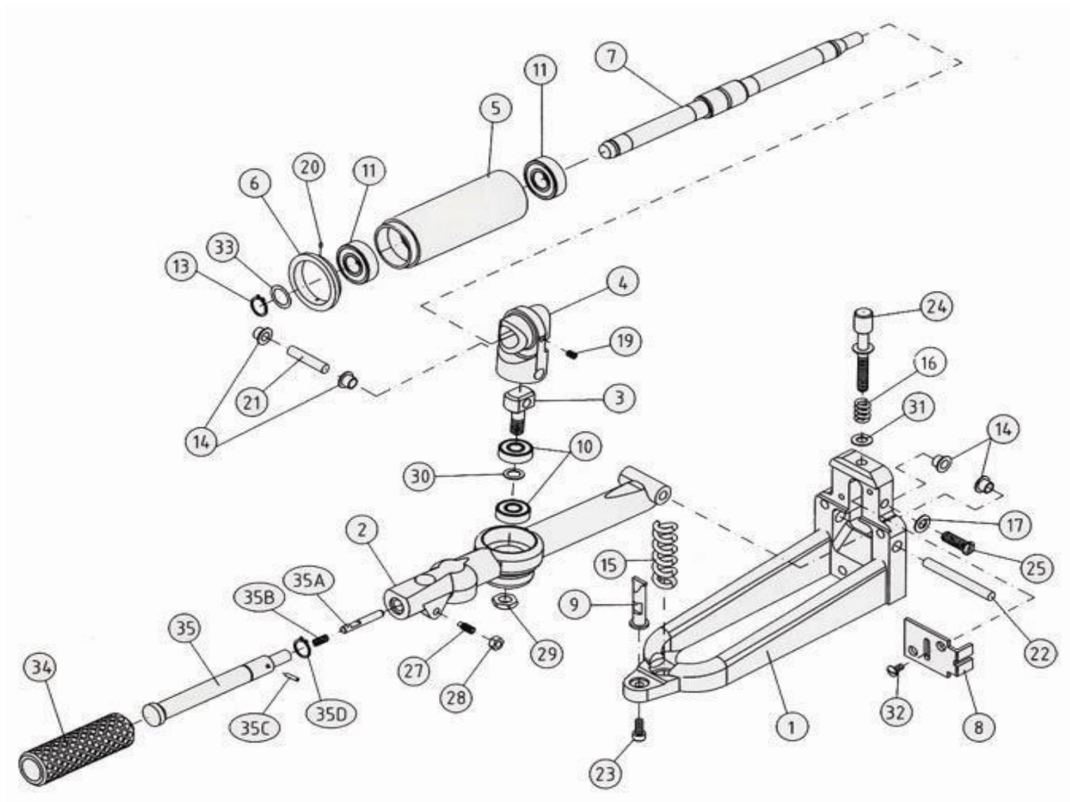
Bona Universal AMO110014.0 Universal tension device 250mm
