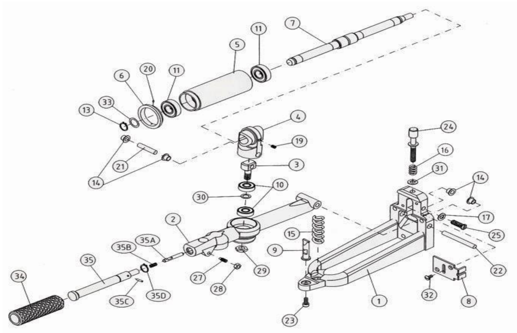
Bona Universal AM0001503 Universal tension device 10"
