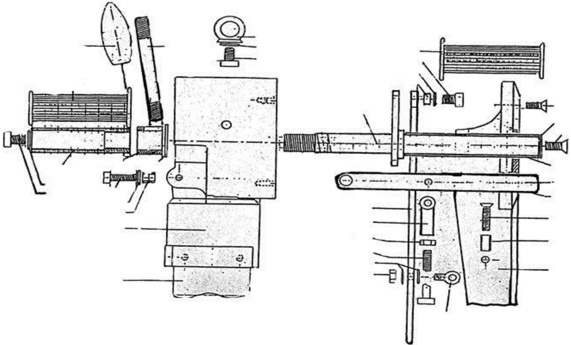
Bona Super 8 Belt Sander AM0001505 Super 8 Feathering Handle
