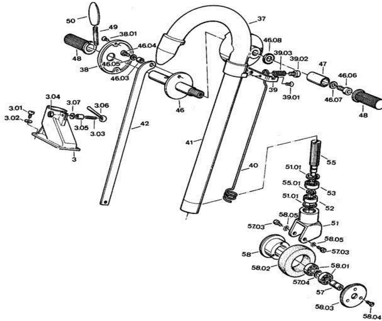
Bona Super 10 Belt Sander AM0001506 Super 10 handle
