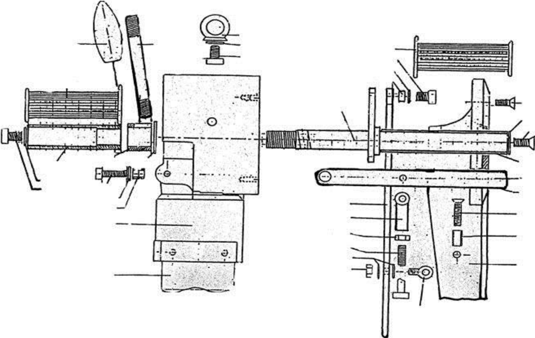
Bona Super 10 Belt Sander AM0001506 Super 10 Feathering handle
