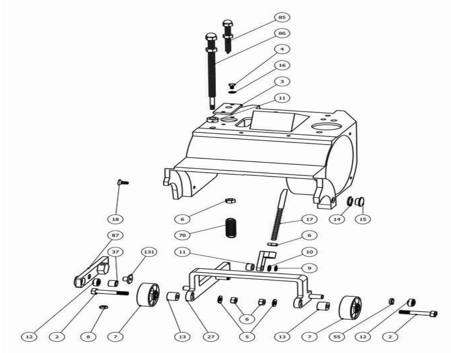
Bona Flexidrum Previous Models AMO150009.3 Flexidrum wheel subframe
