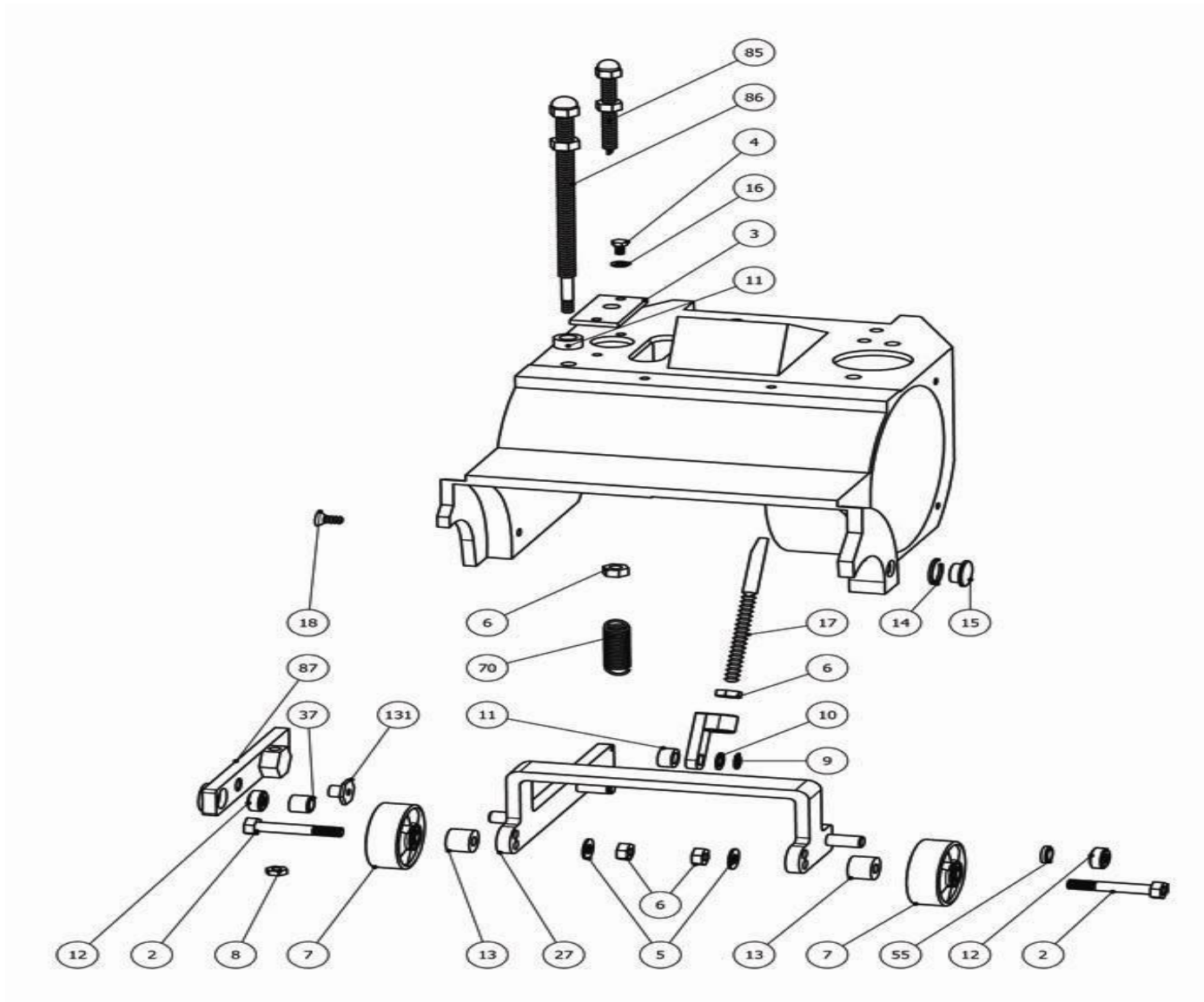
Bona Flexidrum Previous Models AMO150008.3 Flexidrum wheel subframe
