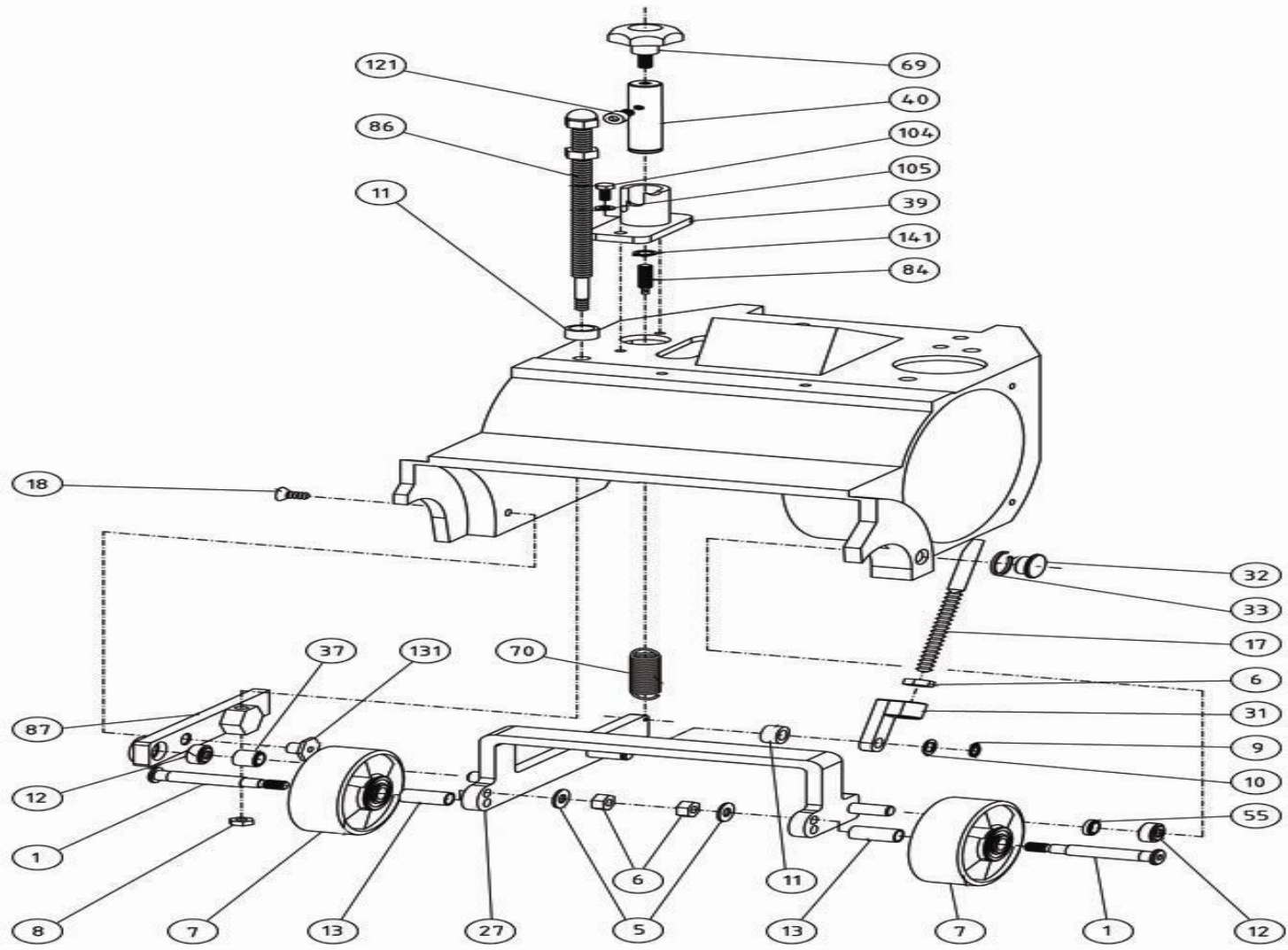
Bona Belt Previous Models AMO110014.3 Belt wheel subframe
