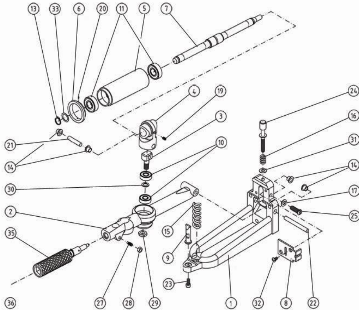
Bona Belt Previous Models AM0003134 Belt Tension device 10"
