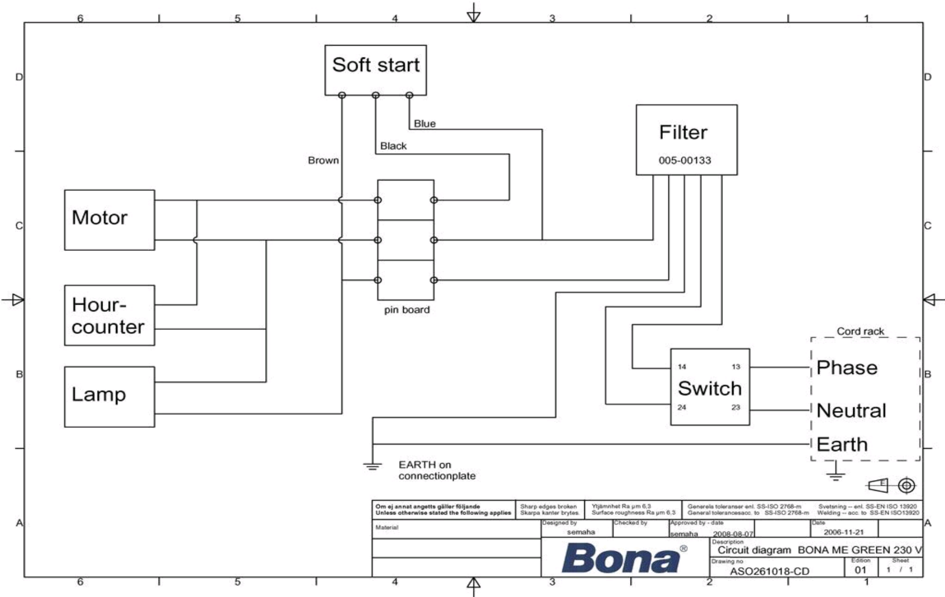
Bona Mini Edge AMO260000.3 El. components 230V Basic Circuit diagram 230V Basic
