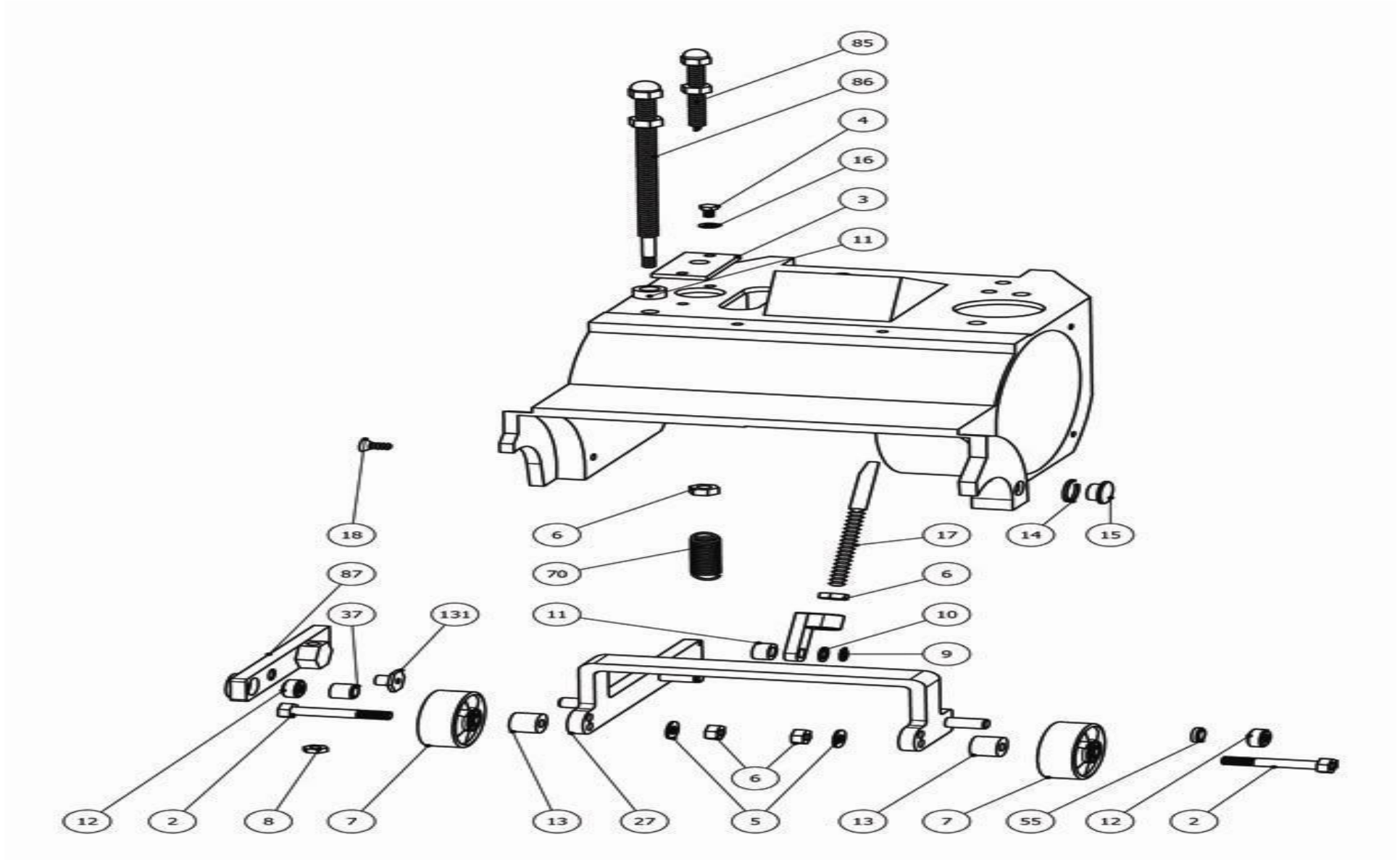
Bona Drum AMO120006.3 Drum wheel subframe
