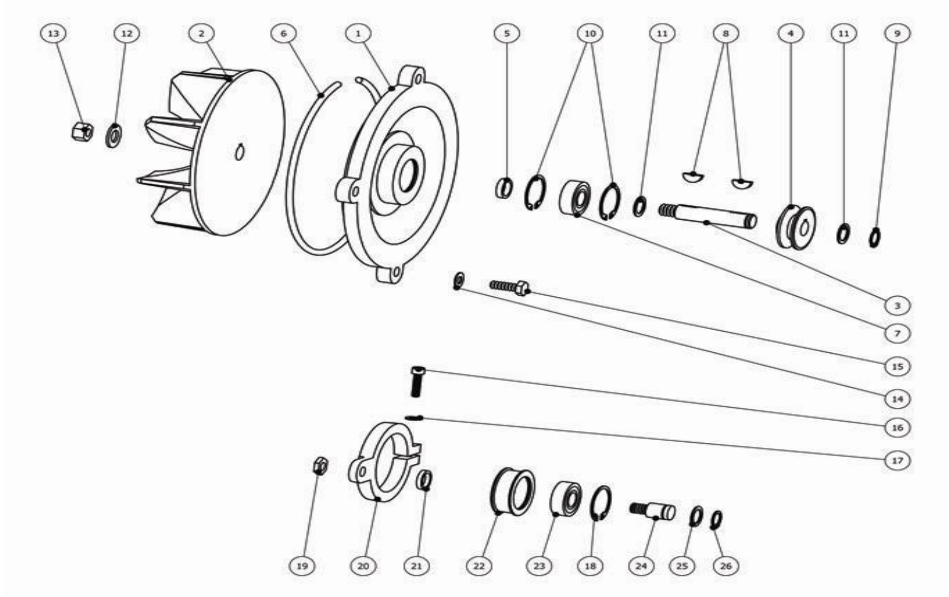
Bona Drum AMO120006.3 Drum Ventilator
