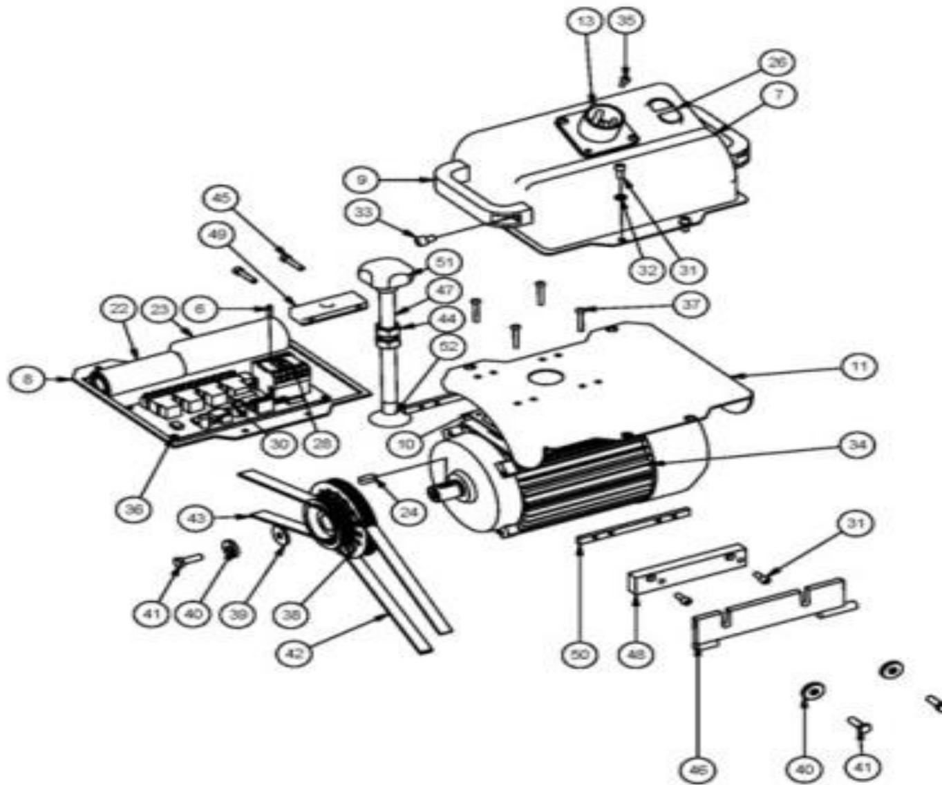
Bona Drum AMO120006.3 Drum Motor 1ph easy start
