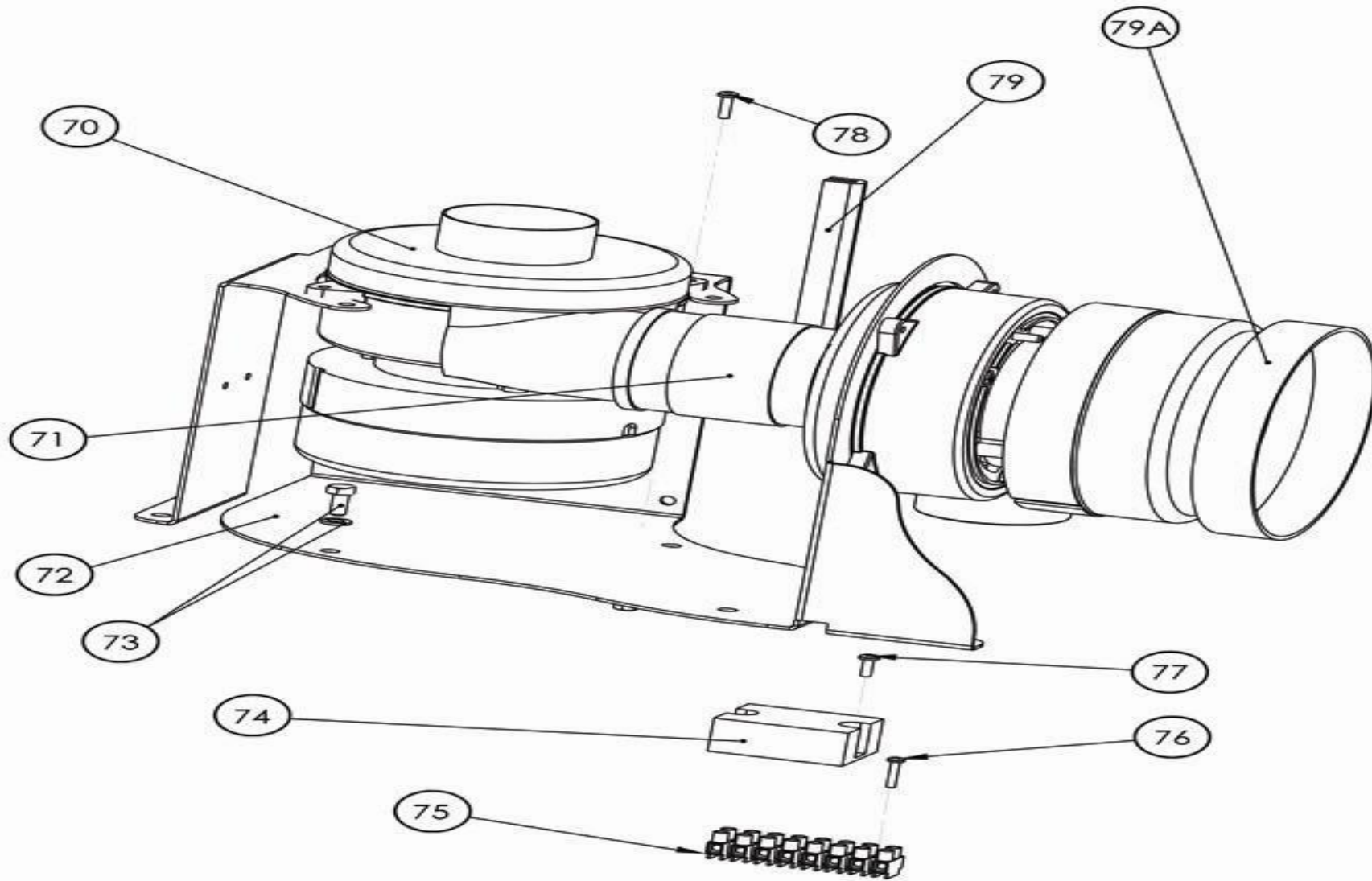
Atomic 110 AD0003401 Vacuum cabinet power pack
