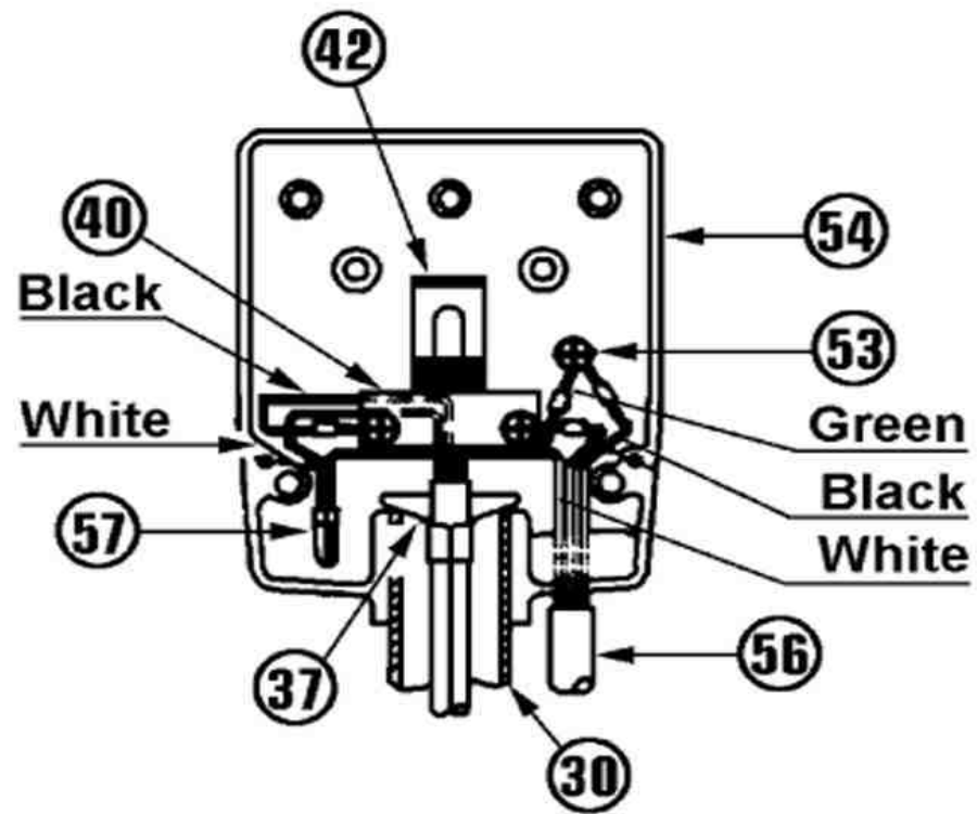
Bona DCS Buffer (old version) AM0001489_DCS Buffer wiring arr._20130415
